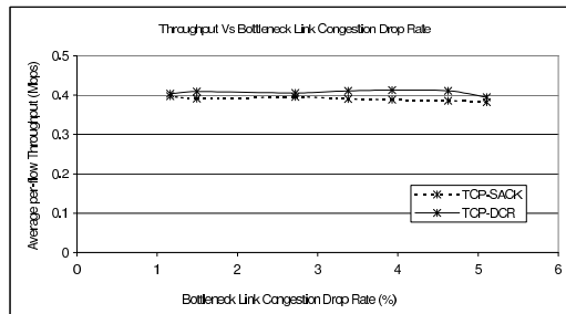
Fig. 10. Throughput Vs Congestion Loss Rate
