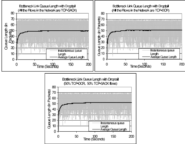
Fig. 15. Bottleneck Link Queue Length with Droptail Queue Management
