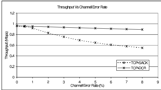
Fig. 5. Throughput Vs Channel Error Rate
