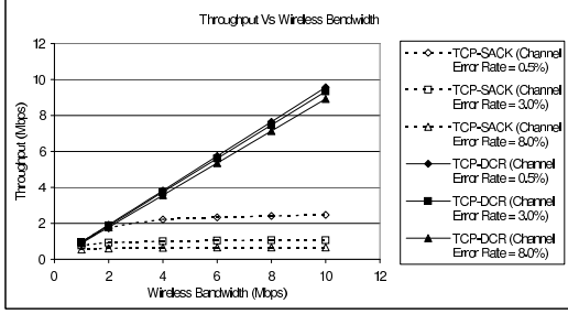
Fig. 7. Throughput Vs Wireless Bandwidth
