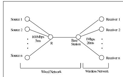
Fig. 9. Network Topology for Experiments with Congestion Losses
