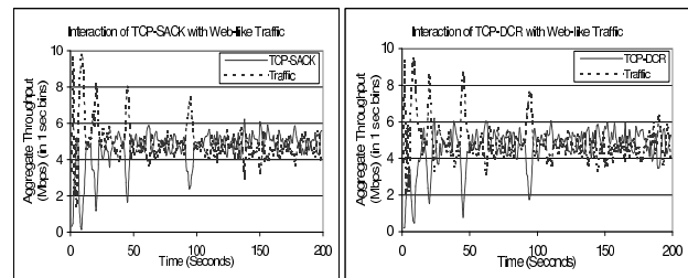
Fig. 12. Interaction with Web-like Traffic
