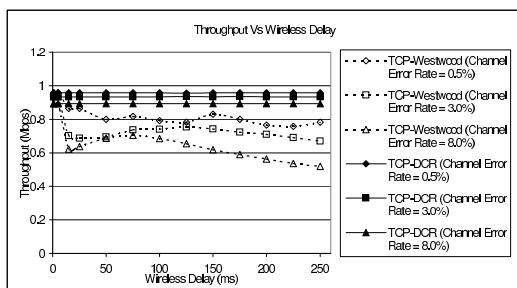
Fig. 20. Performance Comparison of TCP-DCR Vs TCP-Westwood
