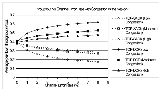
Fig. 18. Throughput Vs Channel Error Rate with Congestion in the Network
