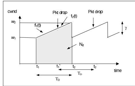
Fig. 3. Analysis of TCP-DCR with no Channel Errors
