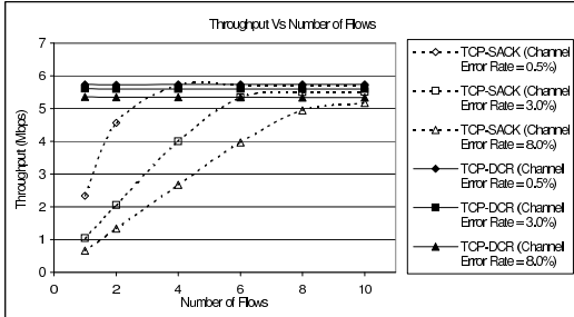
Fig. 8. Throughput Vs Number of Flows
