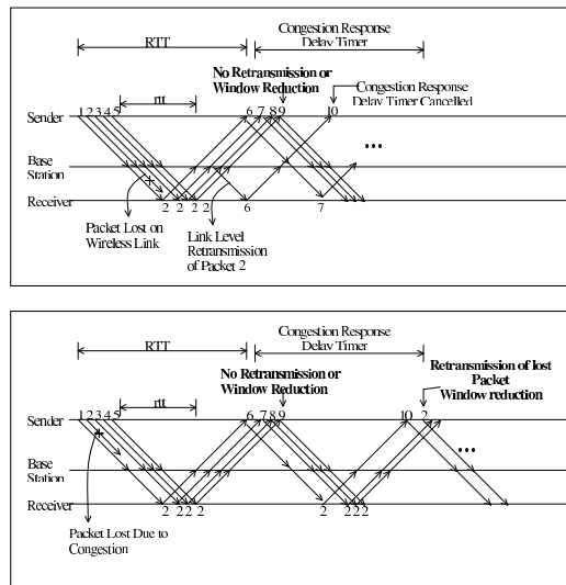
Fig. 1. Behavior of TCP-DCR
