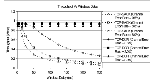
Fig. 6. Throughput Vs Wireless Link Delay
