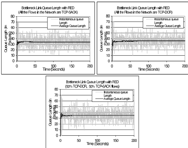
Fig. 16. Bottleneck Link Queue Length with RED Queue Management
