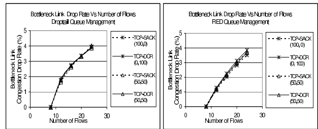
Fig. 17. Bottleneck Link Congestion Loss Rate Vs Number of Flows
