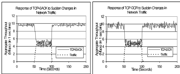
Fig. 11. Throughput Vs Time for Sudden Changes in Traffic
