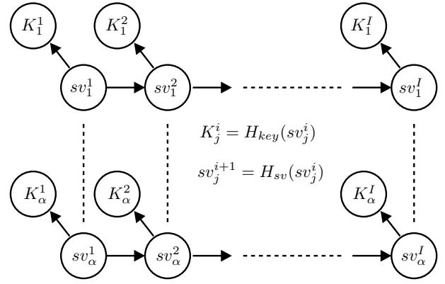
Fig. 8. Key generation from secret values for incremental deployment. K_j^i denotes the j -th key broadcast by a sensor in the i -th initialization phase. H_{key} is a one-way hash function and H_{sv} is a different hash function that is not necessarily one-way.
