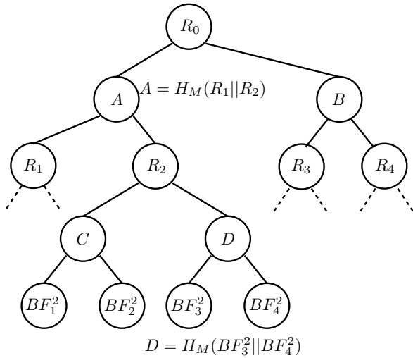
Fig. 9. Two-level Merkle tree for incremental deployment. In this example, there are four sensors and four Bloom filters per sensor for the sets of keys on that device. BF_j^i refers to the Bloom filter for the keys of the i -th sensor for the j -th initialization procedure.
