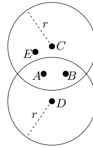
Fig. 2. One-hop neighbors A and B can both overhear broadcasts from C and D . However, C cannot overhear broadcasts from D and vice versa. E is a one-hop neighbor of A , B , and C .
