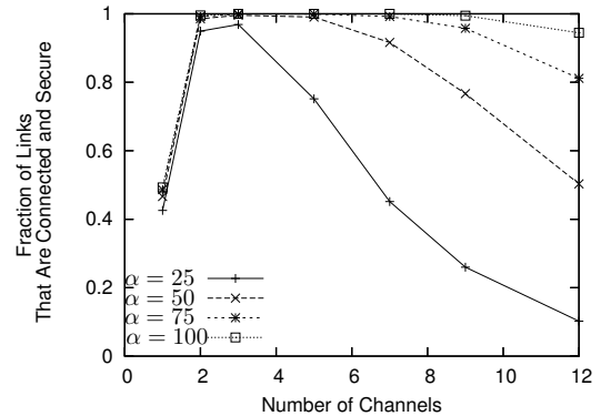
Fig. 6. Secure connectivity of legitimate sensors vs. the number of channels.
