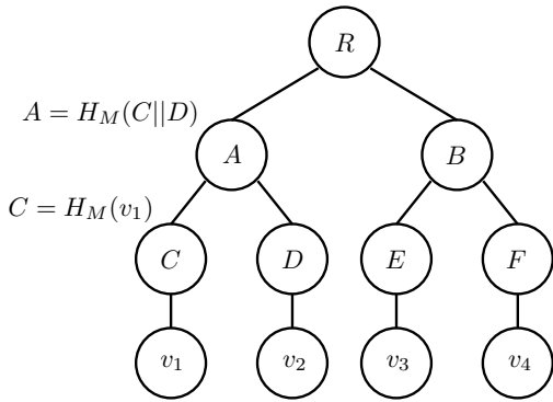
Fig. 1. An example Merkle tree [19] for four objects: v_1, v_2, v_3, v_4 . The leaf nodes are generated by doing a one-way hash, H_M , on the corresponding object. The interior nodes are generated by doing a one-way hash, H_M , on a concatenation of the children of a node.
