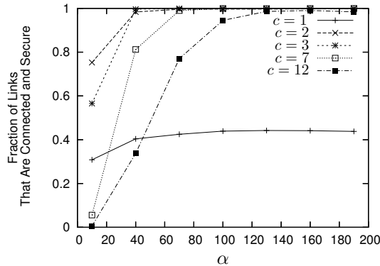
Fig. 4. Secure connectivity of legitimate sensors vs. \alpha .
