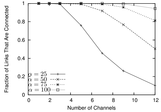
Fig. 5. Connectivity of legitimate sensors vs. the number of channels.
