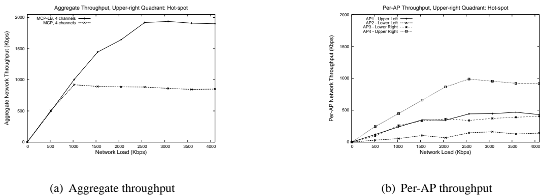
Fig. 9. Aggregate and Per-AP throughput for the scenario with a hot-spot.
