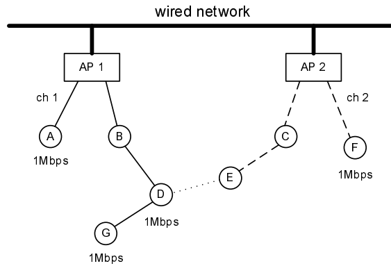
Fig. 3. An example network scenario. This example indicates that subtree load must be considered when selecting the best route.
