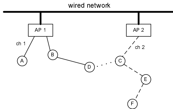
Fig. 2. An example network scenario. This example indicates that number of hops must be considered in measuring the load. The solid lines are links on channel 1, and the dashed lines are links on channel 2.
