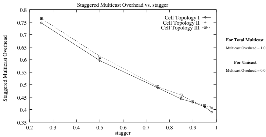
Figure 7: Average Multicast Overhead vs stagger
