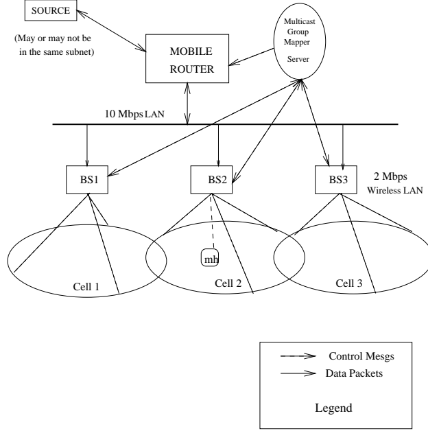
Figure 3: Network Configuration
